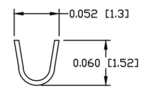
SECTION Y-Y
