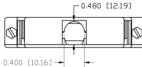
BACK VIEW
